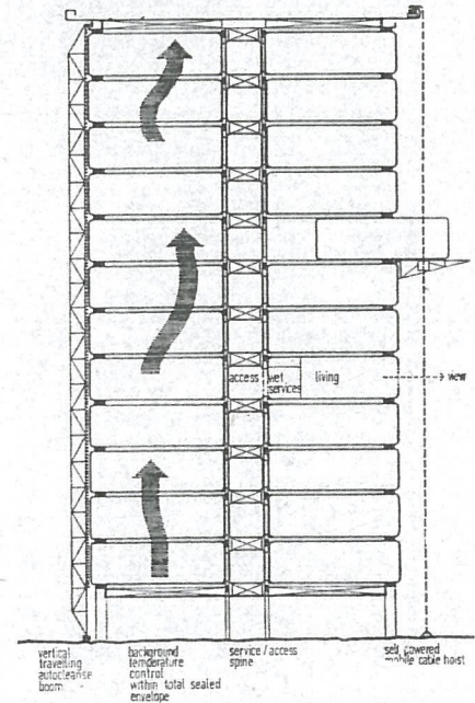
ANALOGISTIC VIEWS showing structural armature and finished capsule
